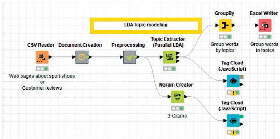
Figure 1 LDA topic modeling KNIME workflow
