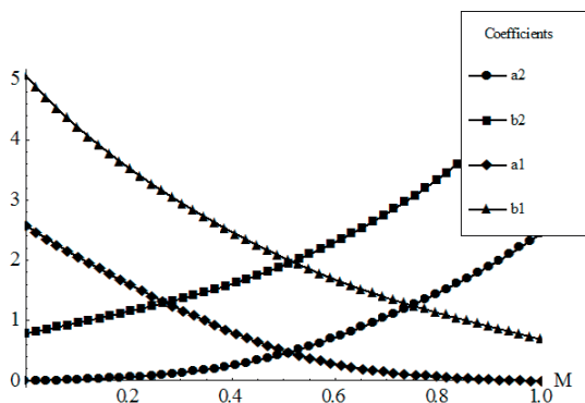
Figure 6 Effects of different costs of offensive and defensive marketing efforts ( \alpha_1=0.6, \alpha_2=0.5, \beta_1=0.4, \beta_2=0.5, \gamma_1=1, \gamma_2=1, c_{11}=c_{21}=1, c_{12}=c_{22}=0.2 )
