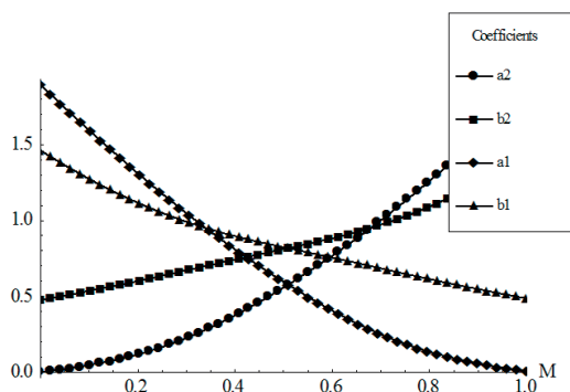
Figure3 Effects of different effectiveness of offensive and defensive marketing efforts ( \alpha_1=0.5, \alpha_2=0.5, \beta_1=0.5, \beta_2=0.5, \gamma_1=1, \gamma_2=1, c_{11}=c_{12}=c_{21}=c_{22}=1 )
