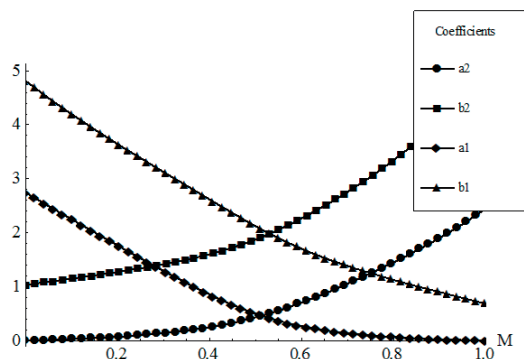
Figure 5 Effects of different costs of offensive and defensive marketing efforts ( \alpha_1=0.75, \alpha_2=0.5, \beta_1=0.25, \beta_2=0.5, \gamma_1=1, \gamma_2=1, c_{11}=c_{21}=1, c_{12}=c_{22}=0.2 )
