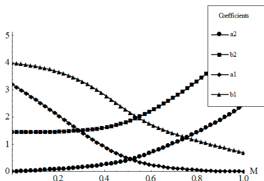
Figure 4 Effects of different costs of offensive and defensive marketing efforts ( \alpha_1=0.9, \alpha_2=0.5, \beta_1=0.1, \beta_2=0.5, \gamma_1=1, \gamma_2=1, c_{11}=c_{21}=1, c_{12}=c_{22}=0,2 )
