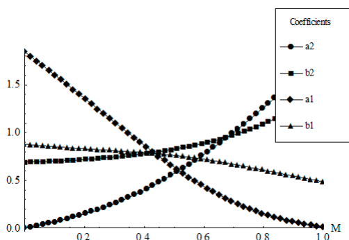
Figure1 Effects of different effectiveness of offensive and defensive marketing efforts ( \alpha_1=0.9, \alpha_2=0.5, \beta_1=0.1, \beta_2=0.5, \gamma_1=1, \gamma_2=1, c_{11}=c_{12}=c_{21}=c_{22}=1 )
